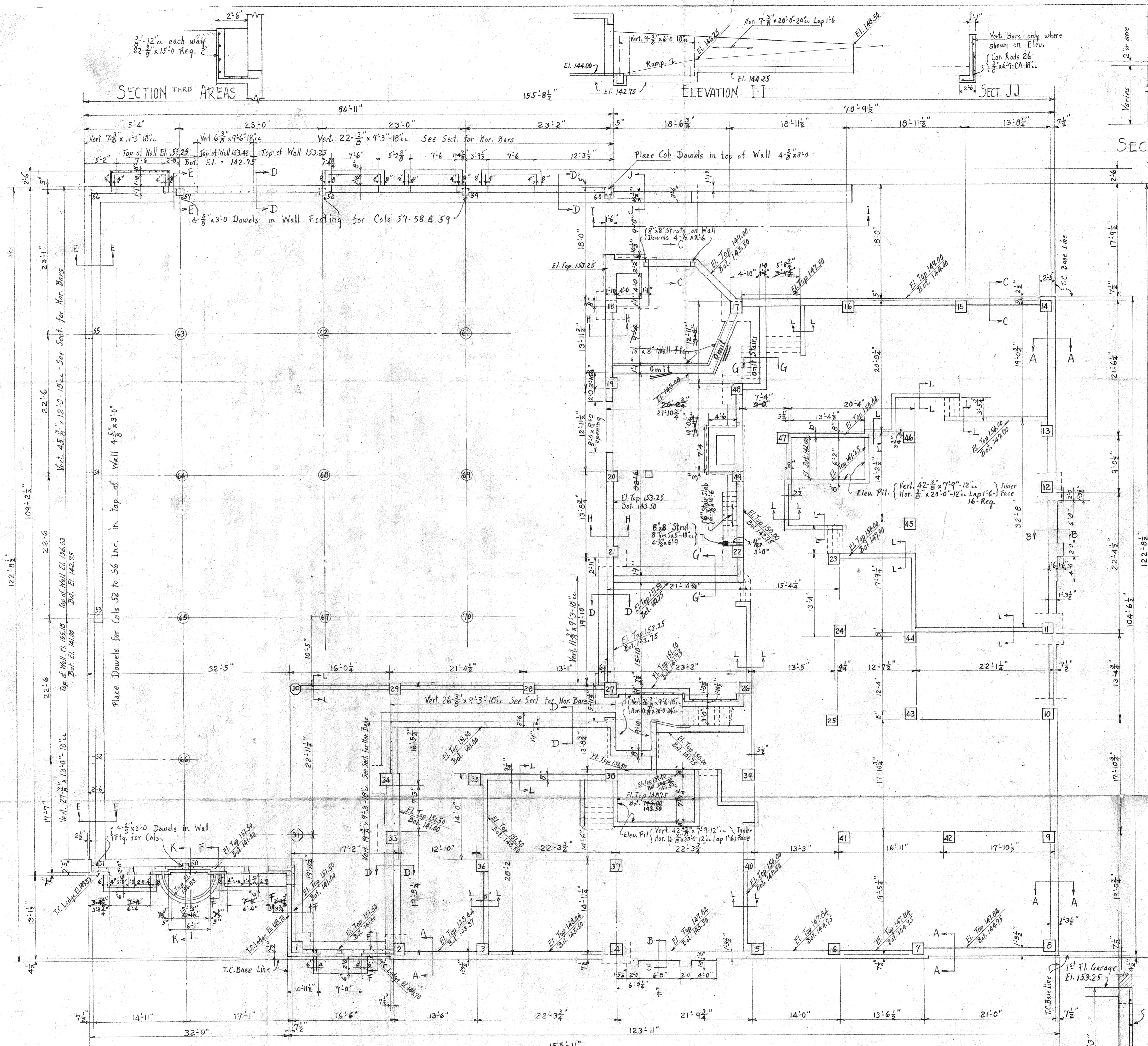
FOUNDATION WALL PLAN Scale: 1/8" = 1'-0"
